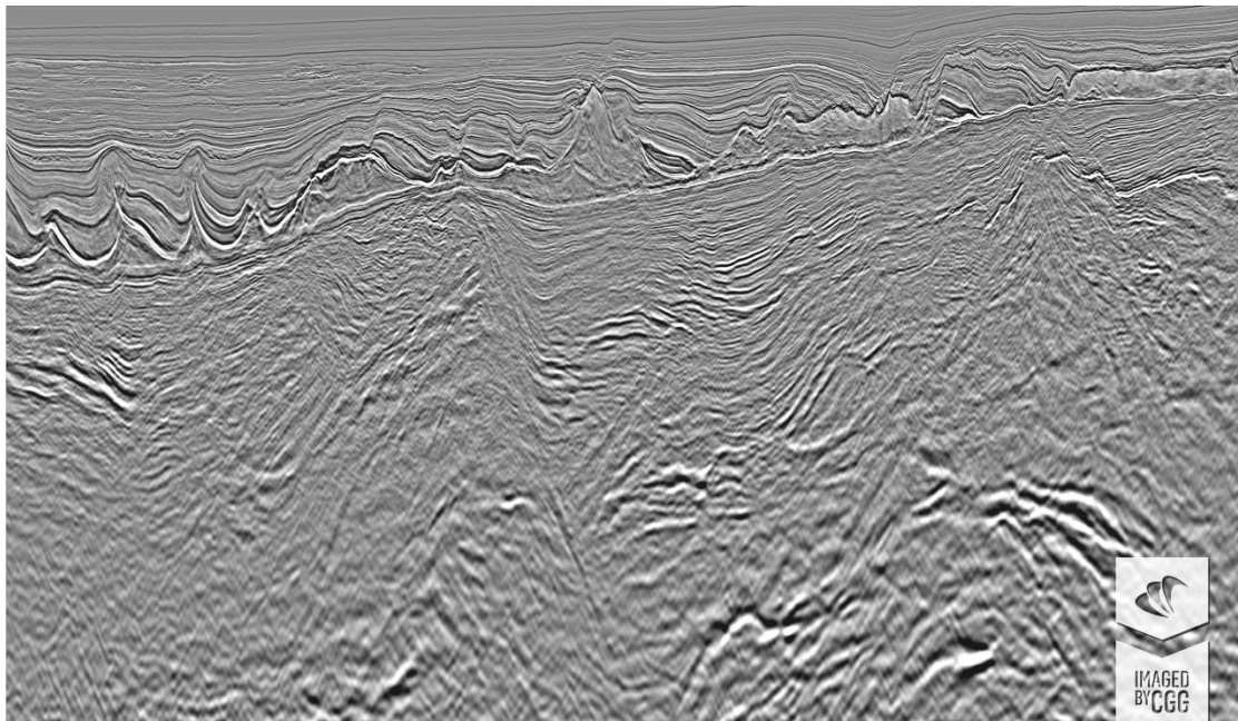
Final Kirchhoff PreSDM image showing a deep pre-salt half-graben with sediments imaged down to 12 km depth and prospective structures at base salt level (Image courtesy of CGG Multi-Client & New Ventures).
